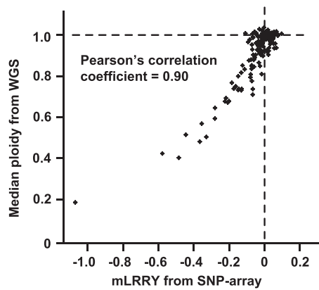
Figure 1. Reproducible Estimations of LOY via Two Independent Technologies
