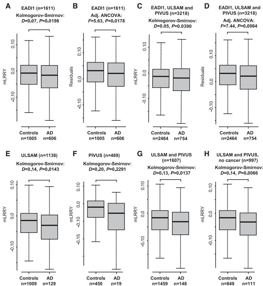
Figure 3. Men Diagnosed with Alzheimer Disease Had on Average a Higher Level of LOY in Blood Cells Compared to AD-free Controls
