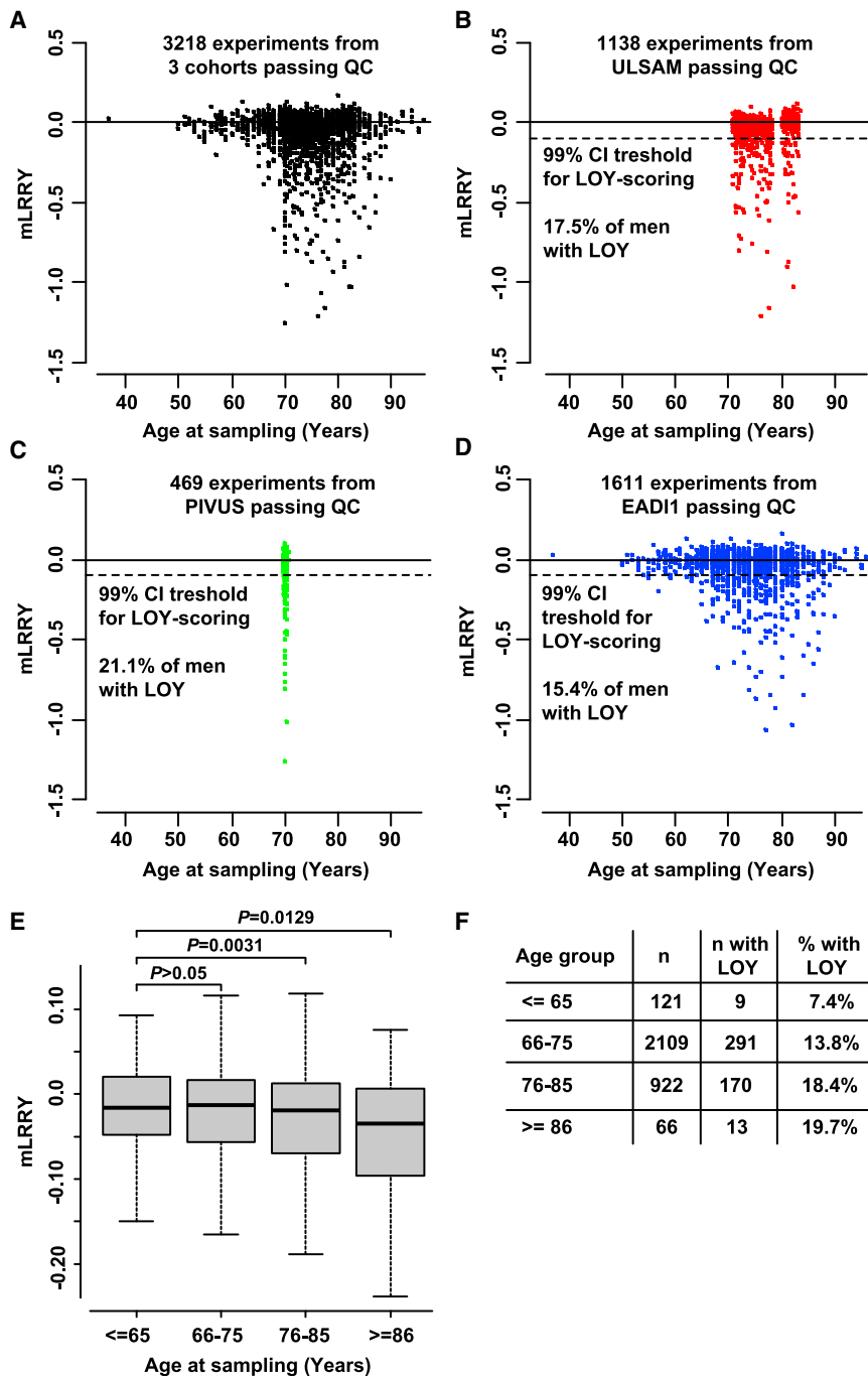
Figure 2. Mosaic LOY in Blood Cells Increases with Participant Sampling Age
