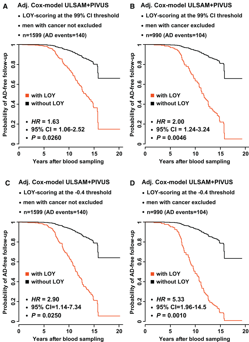
Figure 4. Cox Proportional Hazards Regression Models Adjusting for Potential Confounders Show that Men with Mosaic LOY at Blood Cells at Time for Sampling Were More Likely to Be Diagnosed with AD during the Follow-up Time
